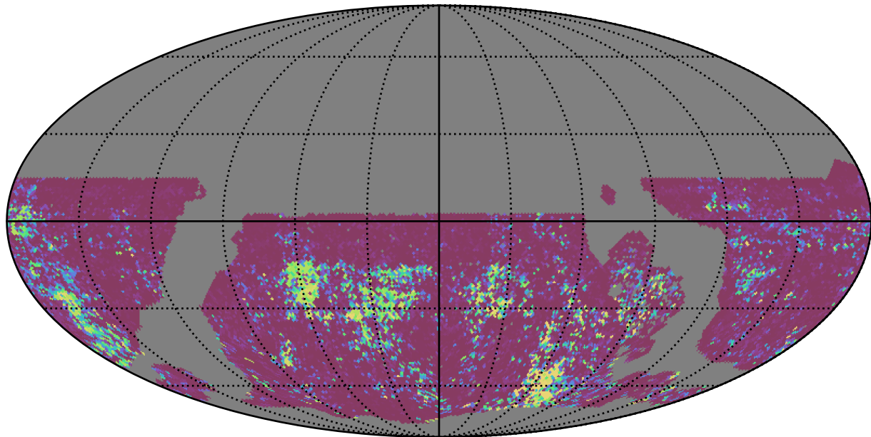
roll_uniform_early_half_accordion1_mjdp0_v3.4_10yrs WFD u band: 75th Percentile Intranight Timespan
