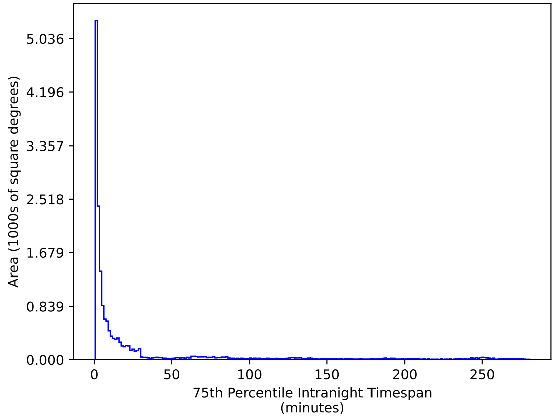
roll_uniform_early_half_accordion1_mjdp0_v3.4_10yrs WFD u band: 75th Percentile Intranight Timespan
