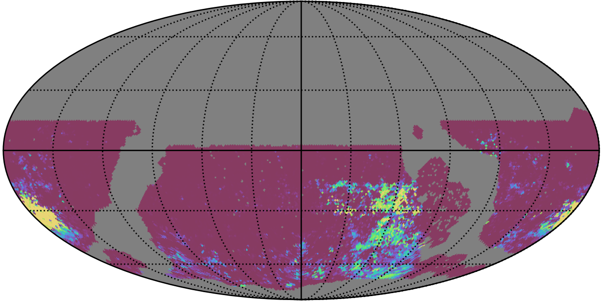
roll_uniform_early_half_accordion1_mjdp0_v3.4_10yrs WFD ri bands: 75th Percentile Intranight Timespan
