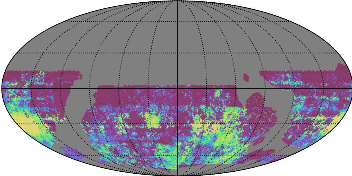
roll_uniform_early_half_accordion1_mjdp0_v3.4_10yrs WFD r band: 75th Percentile Intranight Timespan
