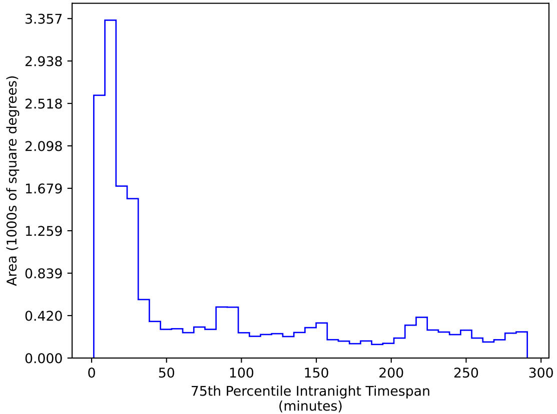
roll_uniform_early_half_accordion1_mjdp0_v3.4_10yrs WFD r band: 75th Percentile Intranight Timespan
