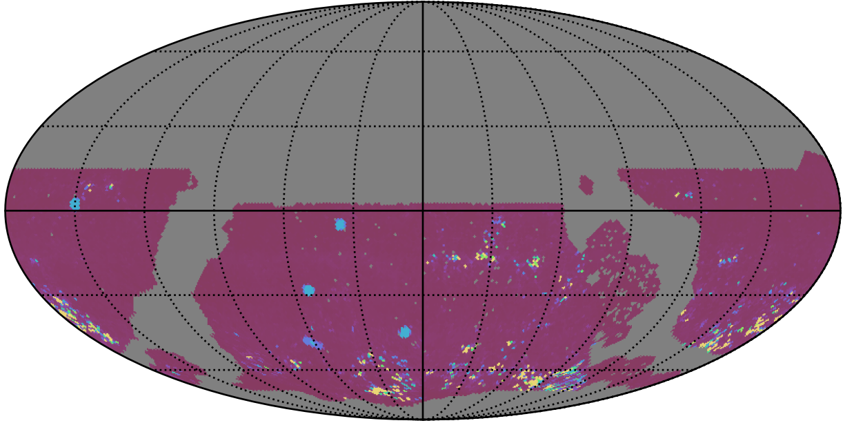
roll_uniform_early_half_accordion1_mjdp0_v3.4_10yrs WFD iz bands: 75th Percentile Intranight Timespan
