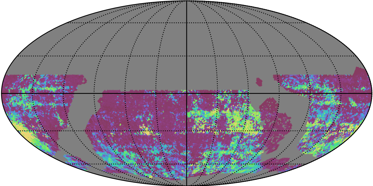
roll_uniform_early_half_accordion1_mjdp0_v3.4_10yrs WFD i band: 75th Percentile Intranight Timespan
