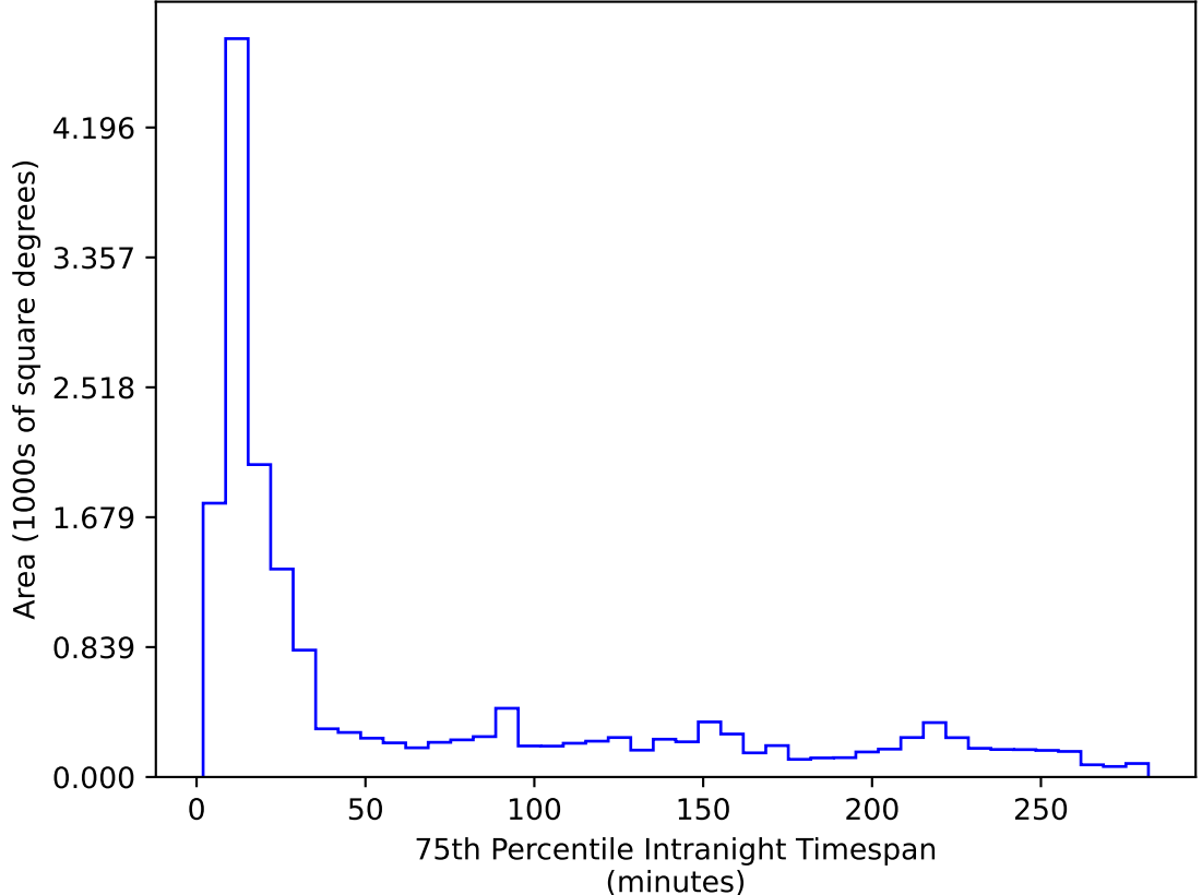
roll_uniform_early_half_accordion1_mjdp0_v3.4_10yrs WFD i band: 75th Percentile Intranight Timespan
