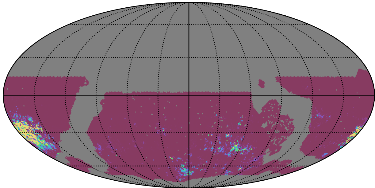
roll_uniform_early_half_accordion1_mjdp0_v3.4_10yrs WFD gr bands: 75th Percentile Intranight Timespan
