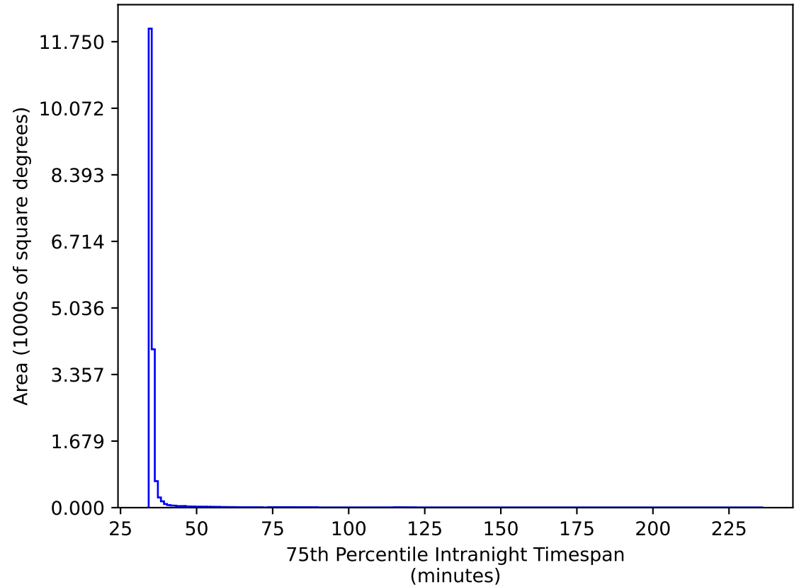
roll_uniform_early_half_accordion1_mjdp0_v3.4_10yrs WFD gr bands: 75th Percentile Intranight Timespan
