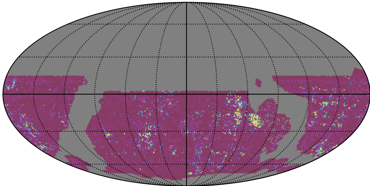
roll_uniform_early_half_accordion1_mjdp0_v3.4_10yrs WFD g band: 75th Percentile Intranight Timespan
