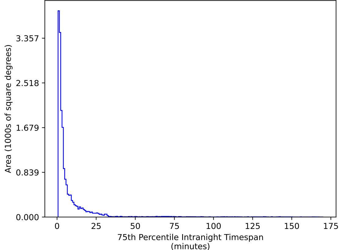
roll_uniform_early_half_accordion1_mjdp0_v3.4_10yrs WFD g band: 75th Percentile Intranight Timespan
