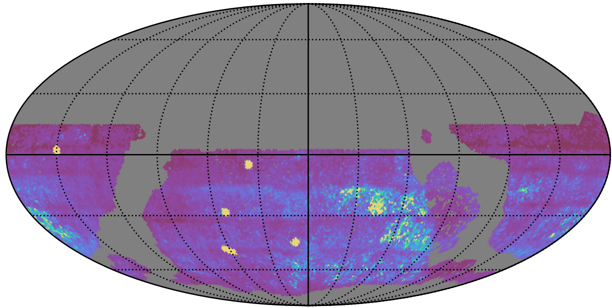
roll_uniform_early_half_accordion1_mjdp0_v3.4_10yrs WFD all bands: 75th Percentile Intranight Timespan
