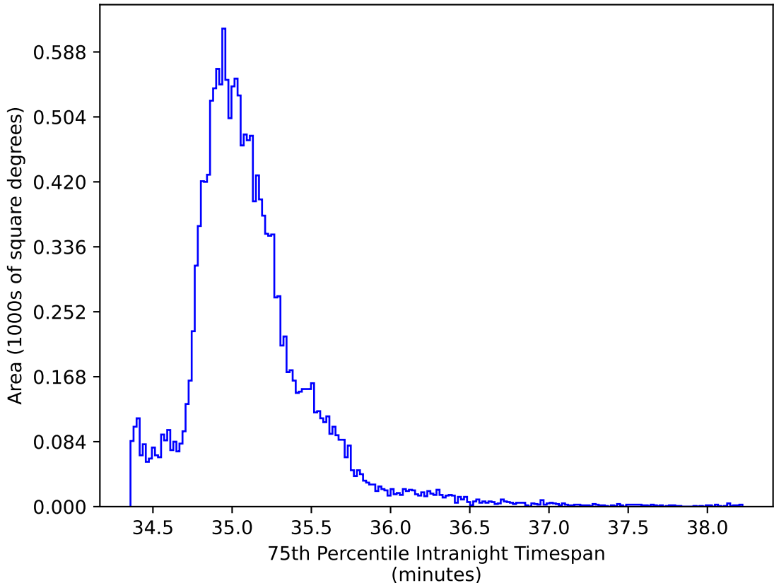
roll_uniform_early_half_accordion1_mjdp0_v3.4_10yrs WFD all bands: 75th Percentile Intranight Timespan
