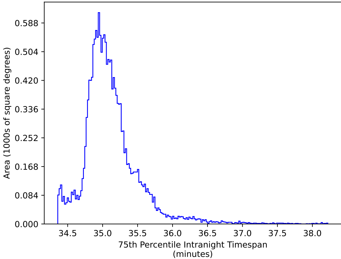
roll_uniform_early_half_accordion1_mjdp0_v3.4_10yrs WFD: 75th Percentile Intranight Timespan
