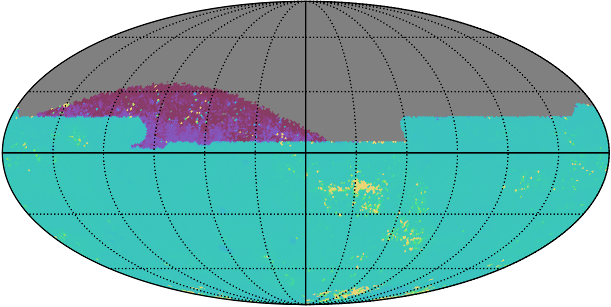
roll_uniform_early_half_accordion1_mjdp0_v3.4_10yrs All sky zy bands: 75th Percentile Intranight Timespan
