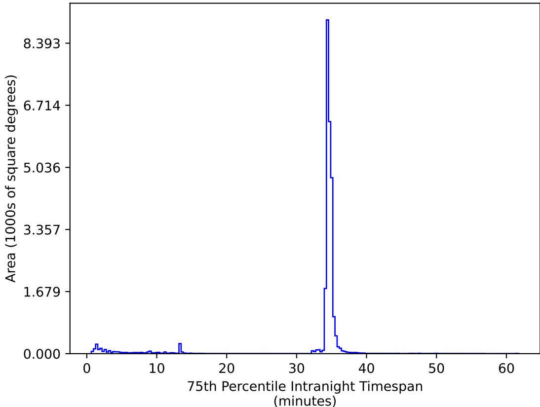
roll_uniform_early_half_accordion1_mjdp0_v3.4_10yrs All sky zy bands: 75th Percentile Intranight Timespan
