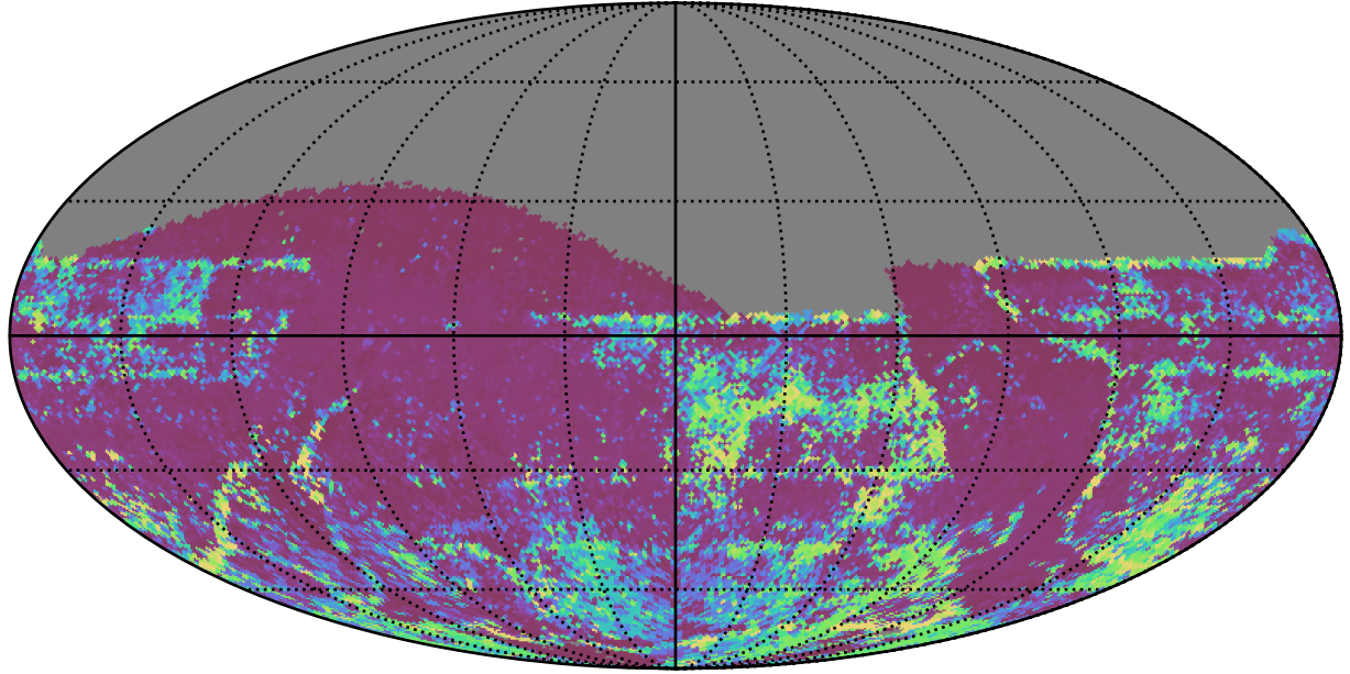
roll_uniform_early_half_accordion1_mjdp0_v3.4_10yrs All sky z band: 75th Percentile Intranight Timespan
