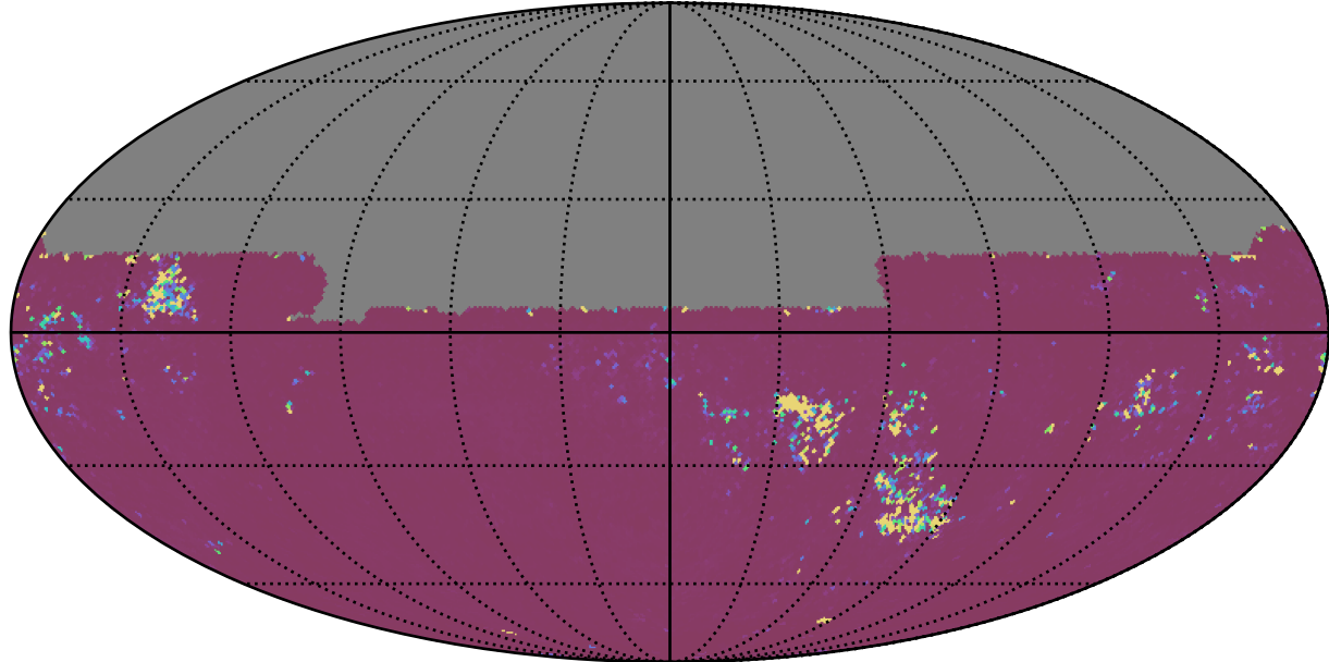
roll_uniform_early_half_accordion1_mjdp0_v3.4_10yrs All sky y band: 75th Percentile Intranight Timespan
