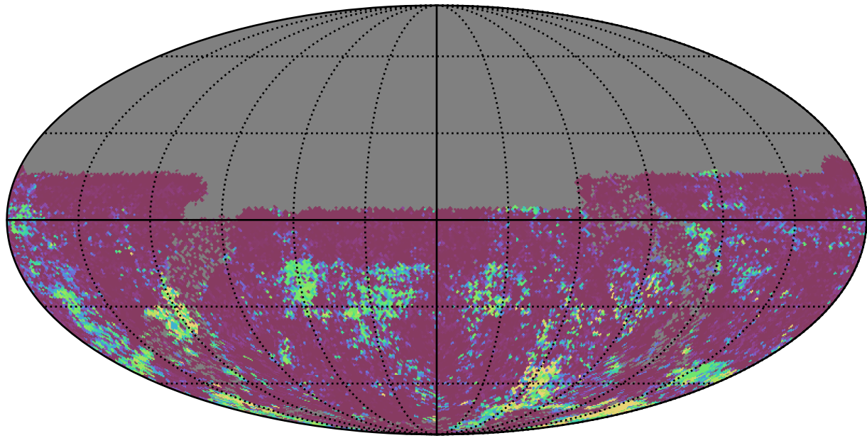
roll_uniform_early_half_accordion1_mjdp0_v3.4_10yrs All sky u band: 75th Percentile Intranight Timespan
