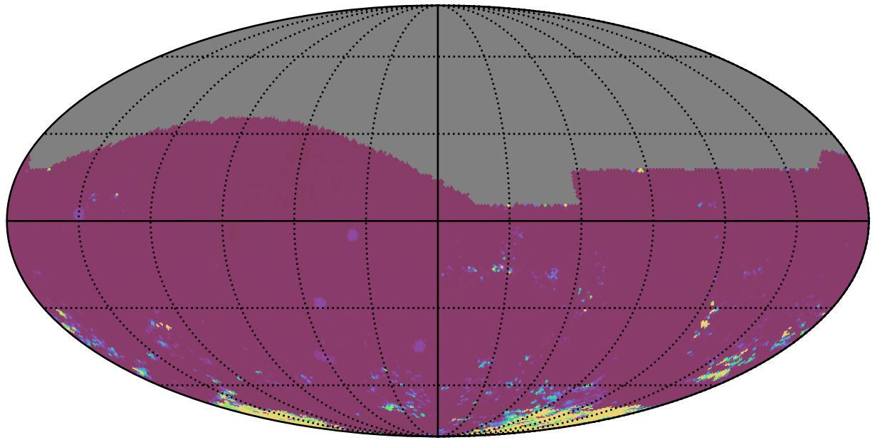
roll_uniform_early_half_accordion1_mjdp0_v3.4_10yrs All sky iz bands: 75th Percentile Intranight Timespan
