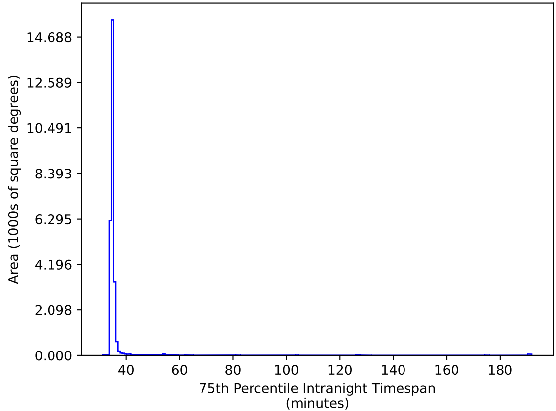
roll_uniform_early_half_accordion1_mjdp0_v3.4_10yrs All sky iz bands: 75th Percentile Intranight Timespan
