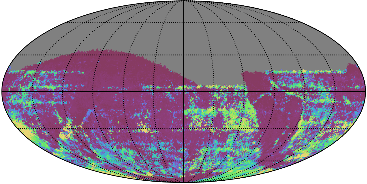
roll_uniform_early_half_accordion1_mjdp0_v3.4_10yrs All sky i band: 75th Percentile Intranight Timespan
