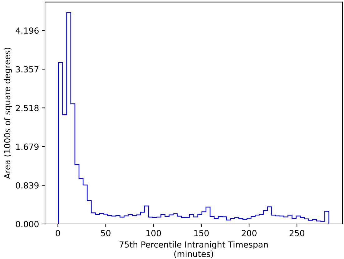
roll_uniform_early_half_accordion1_mjdp0_v3.4_10yrs All sky i band: 75th Percentile Intranight Timespan
