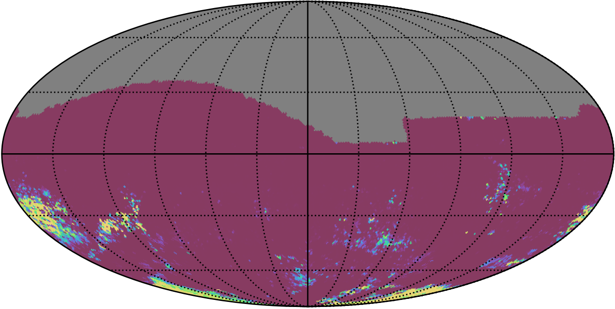
roll_uniform_early_half_accordion1_mjdp0_v3.4_10yrs All sky gr bands: 75th Percentile Intranight Timespan
