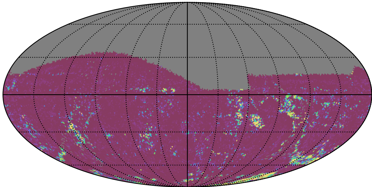
roll_uniform_early_half_accordion1_mjdp0_v3.4_10yrs All sky g band: 75th Percentile Intranight Timespan
