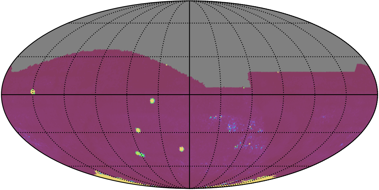
roll_uniform_early_half_accordion1_mjdp0_v3.4_10yrs All sky all bands: 75th Percentile Intranight Timespan
