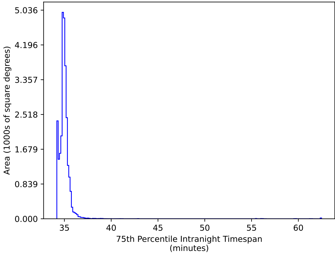
roll_uniform_early_half_accordion1_mjdp0_v3.4_10yrs All sky all bands: 75th Percentile Intranight Timespan
