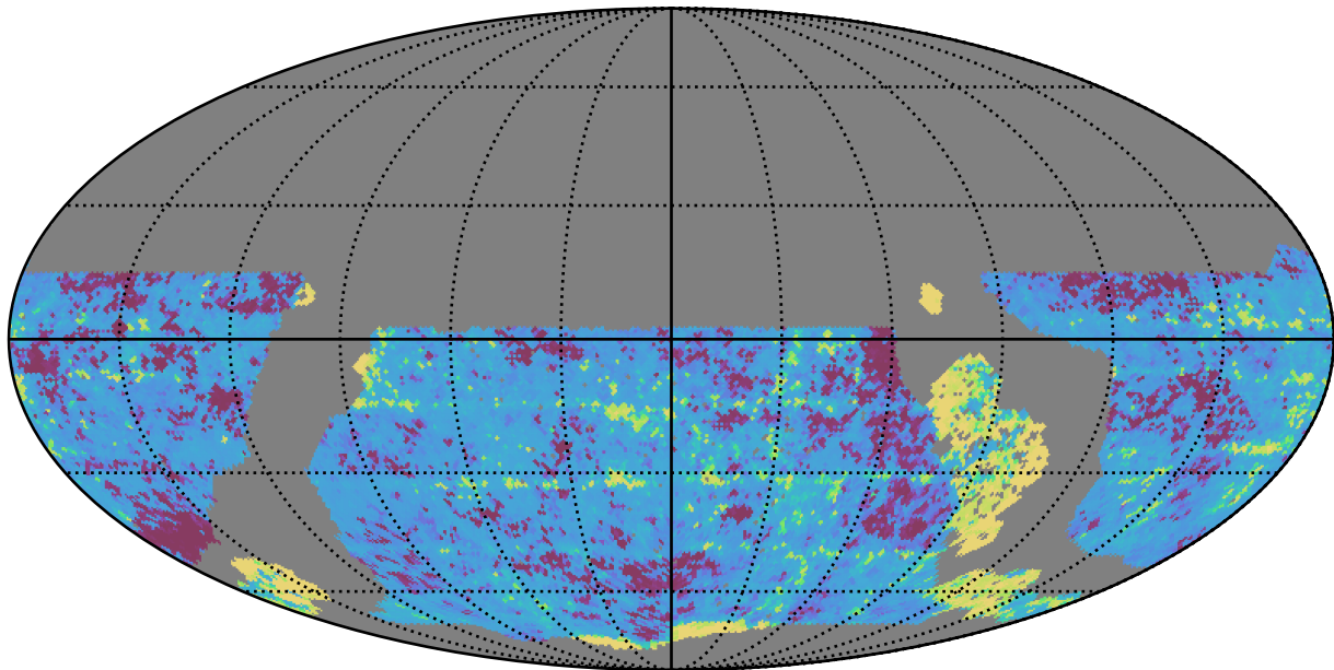
roll_uniform_early_half_accordion1_mjdp0_v3.4_10yrs WFD z band: 20thPercentile Inter-Night Gap
