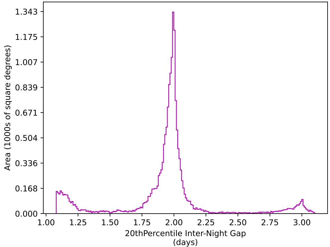
roll_uniform_early_half_accordion1_mjdp0_v3.4_10yrs WFD z band: 20thPercentile Inter-Night Gap
