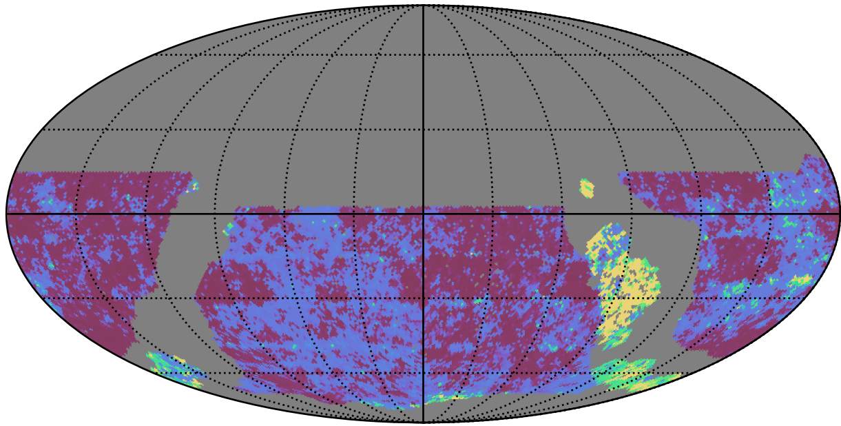
roll_uniform_early_half_accordion1_mjdp0_v3.4_10yrs WFD y band: 20thPercentile Inter-Night Gap
