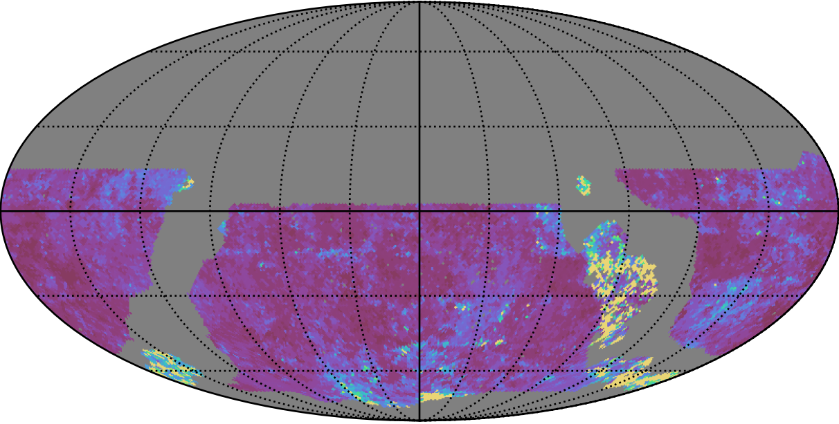
roll_uniform_early_half_accordion1_mjdp0_v3.4_10yrs WFD u band: 20thPercentile Inter-Night Gap
