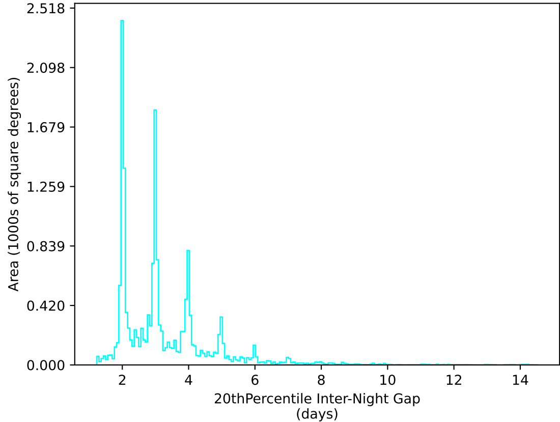
roll_uniform_early_half_accordion1_mjdp0_v3.4_10yrs WFD u band: 20thPercentile Inter-Night Gap
