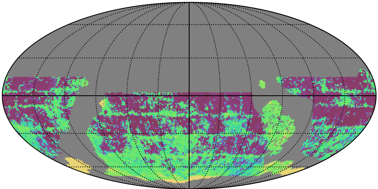
roll_uniform_early_half_accordion1_mjdp0_v3.4_10yrs WFD r band: 20thPercentile Inter-Night Gap
