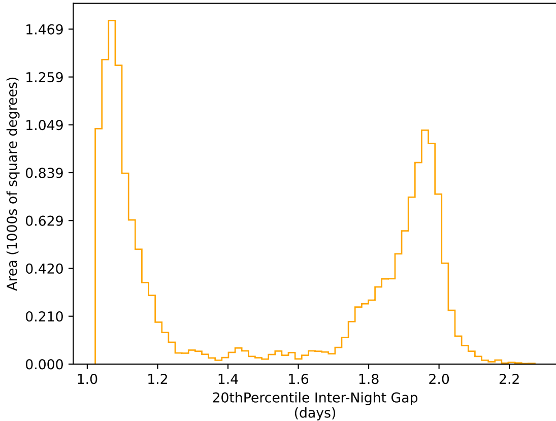
roll_uniform_early_half_accordion1_mjdp0_v3.4_10yrs WFD r band: 20thPercentile Inter-Night Gap
