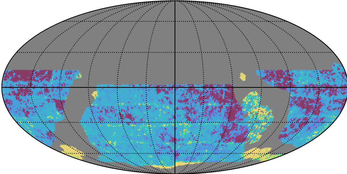
roll_uniform_early_half_accordion1_mjdp0_v3.4_10yrs WFD i band: 20thPercentile Inter-Night Gap
