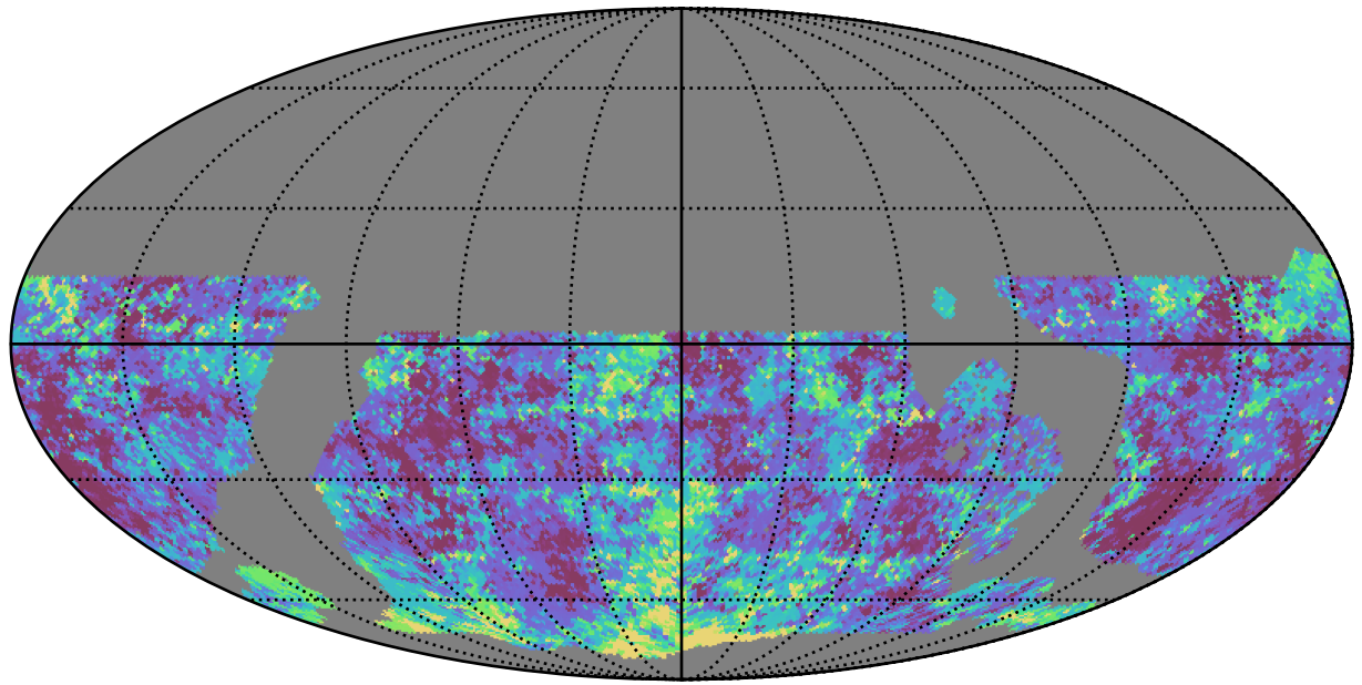
roll_uniform_early_half_accordion1_mjdp0_v3.4_10yrs WFD g band: 20thPercentile Inter-Night Gap
