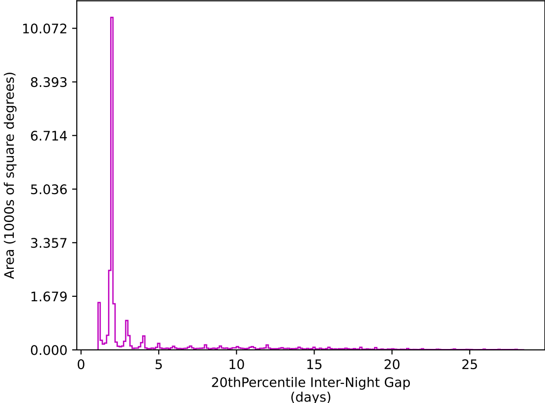
roll_uniform_early_half_accordion1_mjdp0_v3.4_10yrs All sky z band: 20thPercentile Inter-Night Gap
