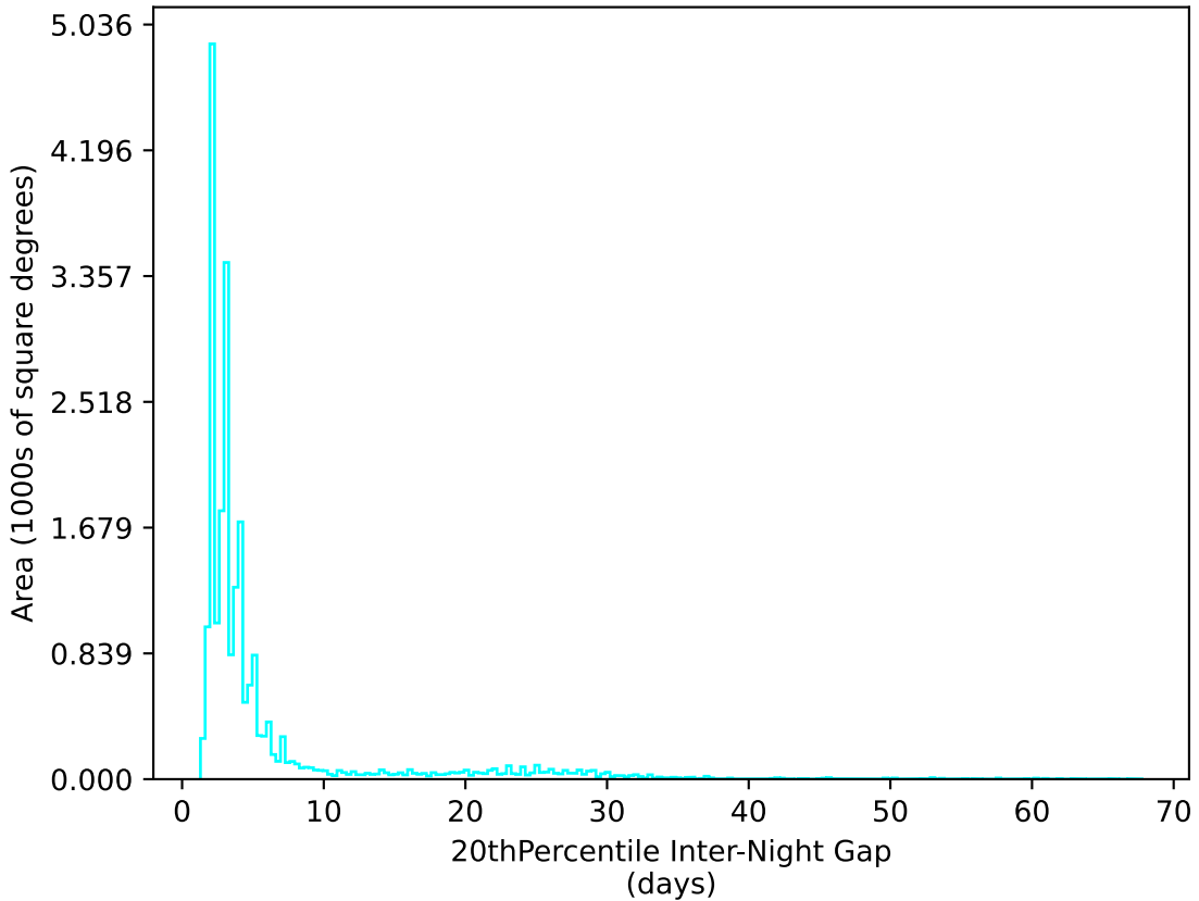
roll_uniform_early_half_accordion1_mjdp0_v3.4_10yrs All sky u band: 20thPercentile Inter-Night Gap
