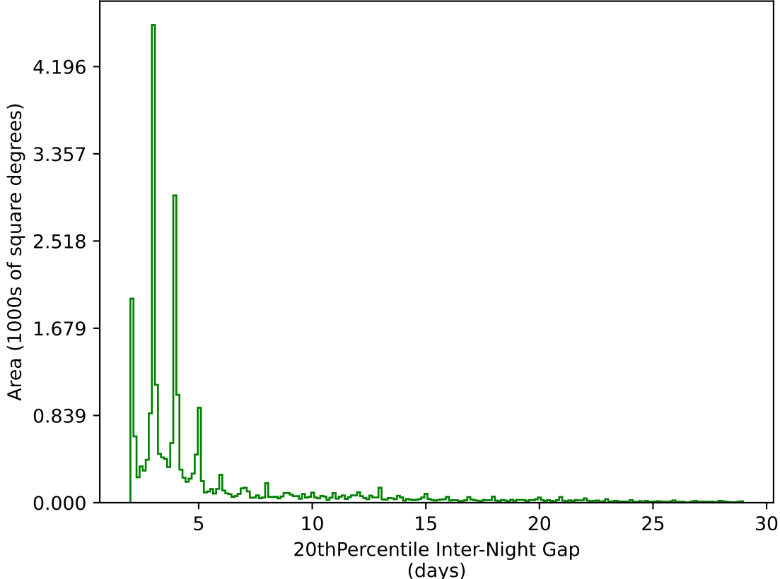
roll_uniform_early_half_accordion1_mjdp0_v3.4_10yrs All sky g band: 20thPercentile Inter-Night Gap
