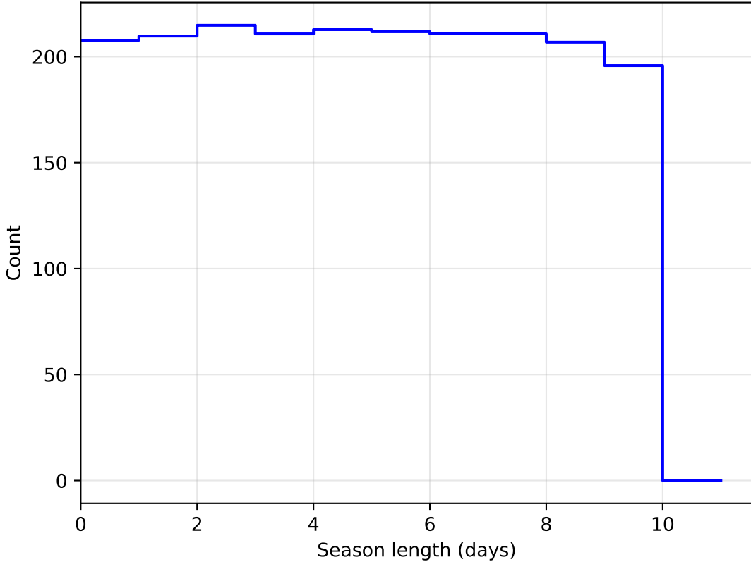
roll_uniform_early_half_accordion1_mjdp0_v3.4_10yrs DD:EDFS all bands: SeasonLength
