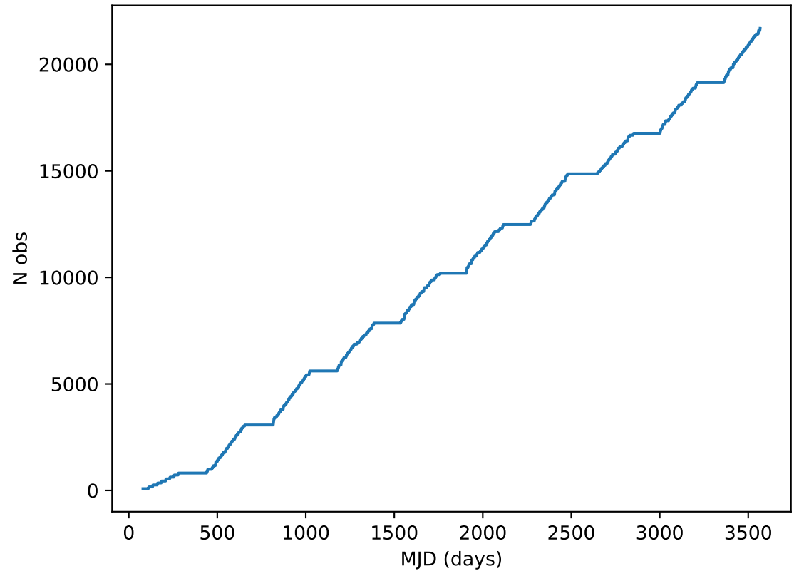
roll_uniform_early_half_accordion1_mjdp0_v3.4_10yrs all bands: DD:XMM_LSS Cumulative NVisits
