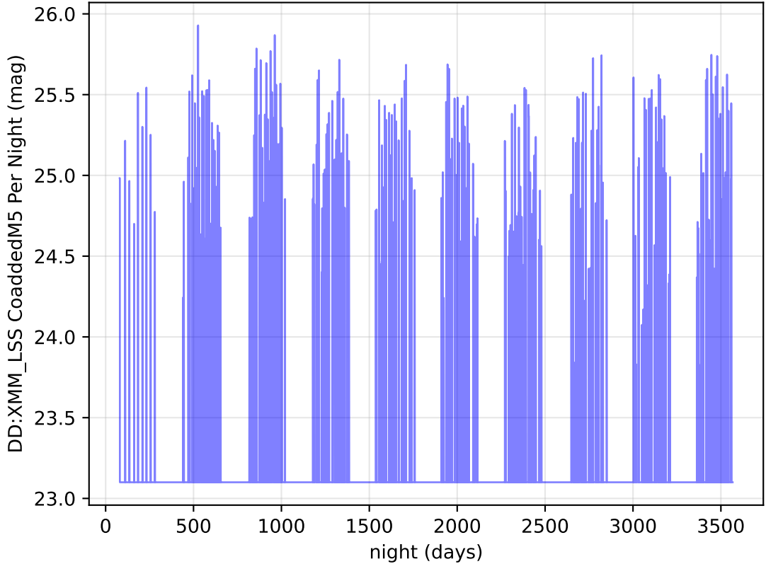
roll_uniform_early_half_accordion1_mjdp0_v3.4_10yrs i band: DD:XMM_LSS CoaddedM5 Per Night
