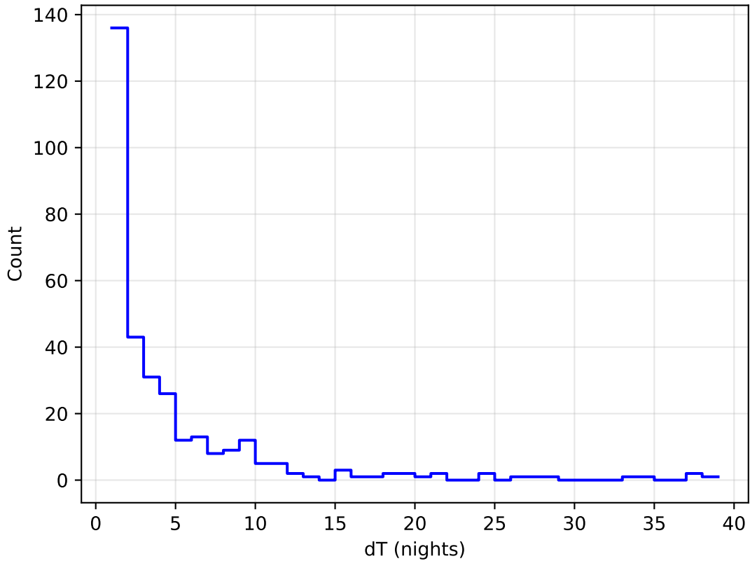
roll_uniform_early_half_accordion1_mjdp0_v3.4_10yrs all bands: DD:WFD Delta Nights Histogram
