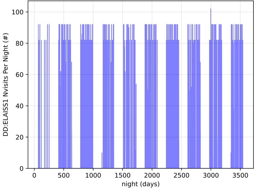
roll_uniform_early_half_accordion1_mjdp0_v3.4_10yrs all bands: DD:ELAISS1 Nvisits Per Night
