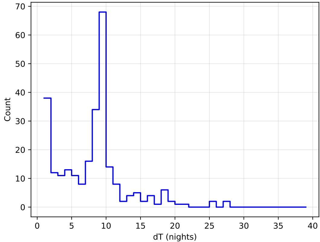
roll_uniform_early_half_accordion1_mjdp0_v3.4_10yrs all bands: DD:ELAISS1 Delta Nights Histogram
