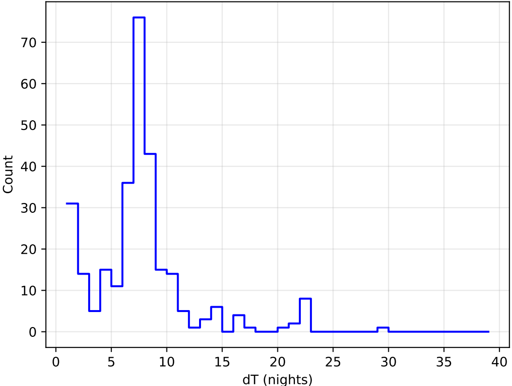
roll_uniform_early_half_accordion1_mjdp0_v3.4_10yrs all bands: DD:EDFS Delta Nights Histogram
