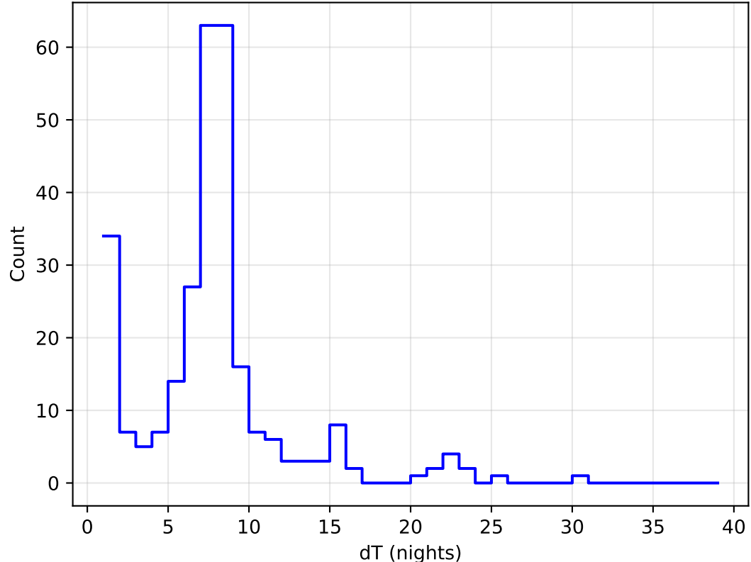
roll_uniform_early_half_accordion1_mjdp0_v3.4_10yrs all bands: DD:ECDFS Delta Nights Histogram
