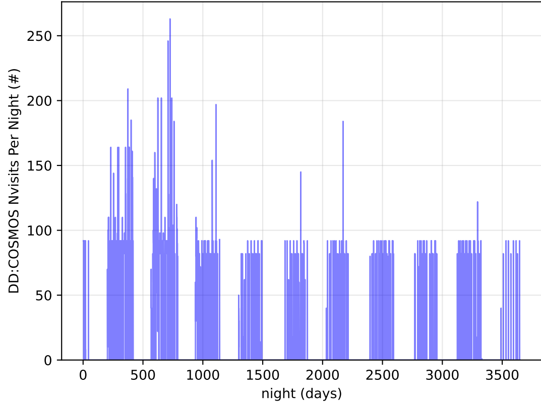
roll_uniform_early_half_accordion1_mjdp0_v3.4_10yrs all bands: DD: COSMOS Nvisits Per Night
