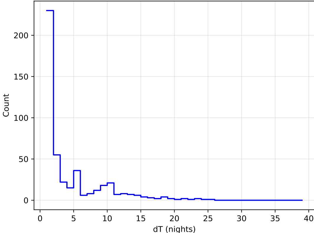
roll_uniform_early_half_accordion1_mjdp0_v3.4_10yrs all bands: DD: COSMOS Delta Nights Histogram
